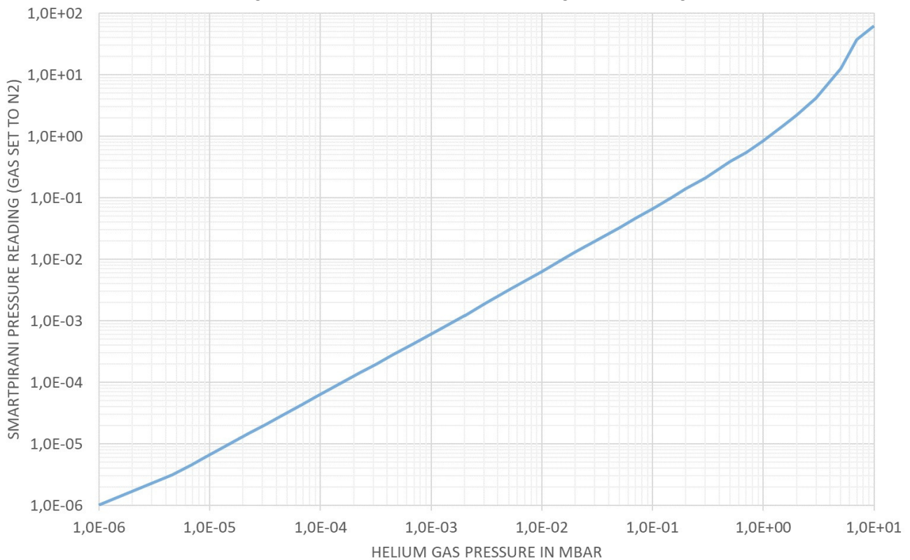
DigiVac Quantum Sensors reading in Helium gas
