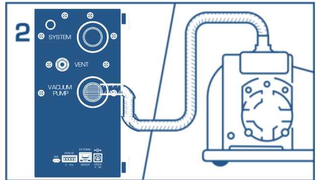
Connect vacuum
